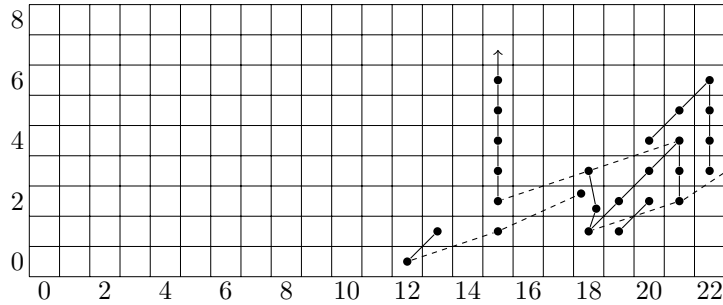
Figure 3: The Adams Spectral Sequence for Q
