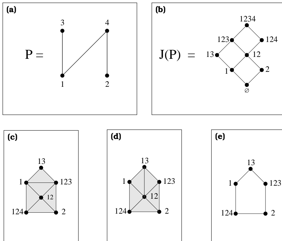
FIGURE 1. (a) A graded poset P . (b) The distributive lattice of order ideals J(P) . (c) Part of the canonical triangulation \Delta J(P) of its order polytope \mathcal{O}(P) . (d) The analogous part of the equatorial triangulation. (e) The equatorial 1-sphere \Delta_{eq}(P) .
