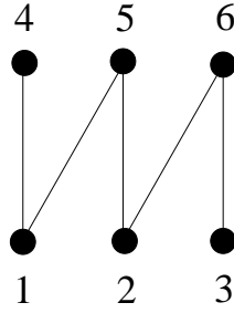
FIGURE 2. Zig-Zag Poset
