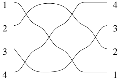
Fig. 8 The alternating scheme
