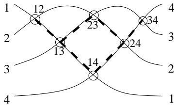
Fig. 7 The natural partial order on the crossings of an arrangement
