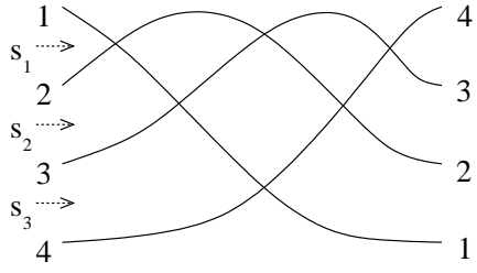
Fig. 5 The arrangement of pseudolines corresponding to s_1 s_2 s_3 s_1 s_2 s_1
