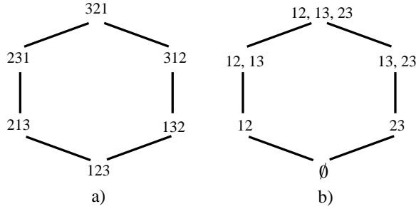
Fig. 1 The weak Bruhat order \mathbb{B}(3, 1)
