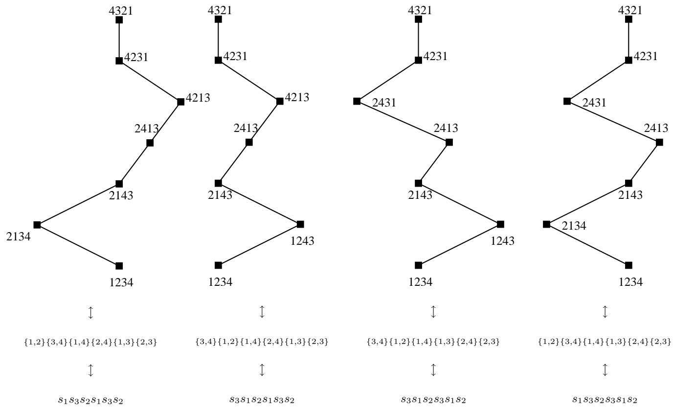
Fig. 3 The correspondences among permutations of \binom{[n]}{2} , maximal chains, and maximal reduced decompositions
