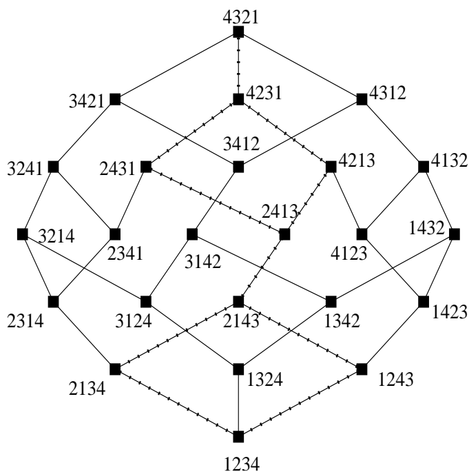
Fig. 2 The weak Bruhat order \mathbb{B}(4, 1)
