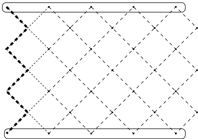
Fig. 16 Representing ideals as paths
