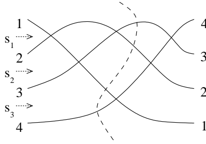
Fig. 6 The permutation corresponding to this new pseudoline is 3214
