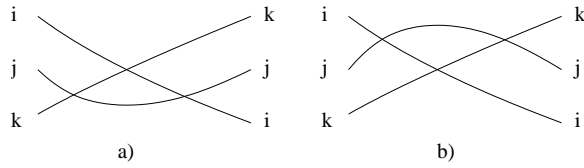
Fig. 4 The set \{i, j, k\} is an inversion in a), but not in b)
