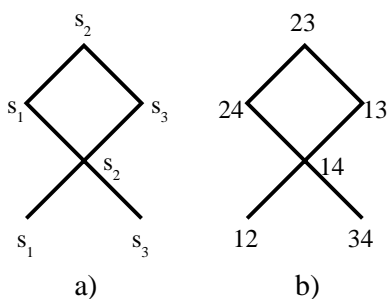
Fig. 12 The natural partial order
