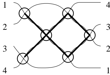
Fig. 11 The natural partial order on the set of crossings
