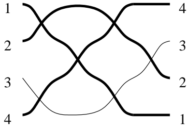
Fig. 10 Strings 1, 2 and 4 make a downward pointing triangle
