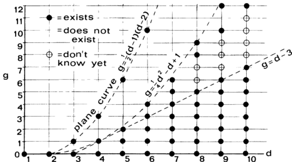
Figure 18. Curves of degree d and genus g in \mathbb{P}^3 .
