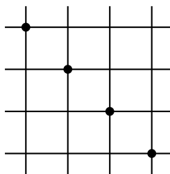
FIGURE 1. A four-point configuration whose minimal free resolution depends on the cross ratio. Each ruling correspond to one copy of \mathbb{P}^1 .
