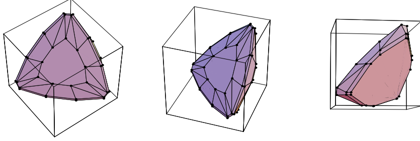
FIGURE 2. Minkowski sum P_1 + P_2 + P'_3 of the Newton polytopes for equations (21)
