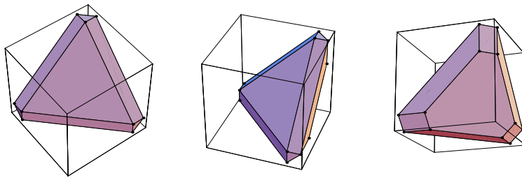
FIGURE 1. The shaded polytope is the Minkowski sum P_1 + P_2 + P_3 of the Newton polytopes for equations (22)
